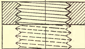
CONVENTIONAL REPRESENTATION
